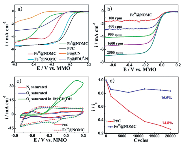
Figure 3. a) RDE voltammetric response for the ORR in O 2 -saturated 0.1 M NaOH at a scan rate of 10 mV s -1 . b) RDE voltammograms recorded for Fe 10 @NOMC electrode in an O 2 -saturated 0.1 M NaOH solution with different rotation rates at a scan rate of 10 mV s -1 . c) CV curves of Fe 10 @NOMC and Pt/C catalysts at a scan rate of 50 mV s -1 in O 2 - or N 2 -saturated 0.1 M NaOH solutions as well as O 2 -saturated 0.1 M NaOH solution with 1 M CH 3 OH. d) Current density degradation at 0 V (vs. Hg/HgO) in the potential cycling process from -0.25 to 0.10 V at a scan rate of 100 mV s -1 .
